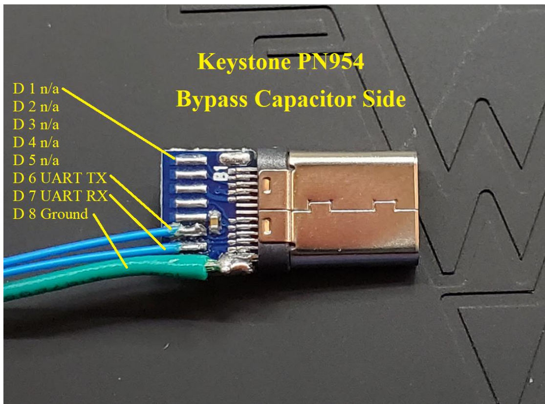
Keystone PN954 Wiring
