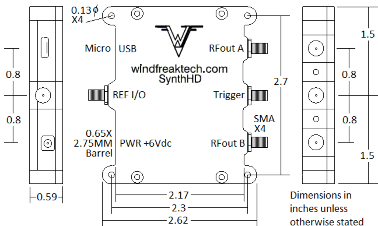
Figure 1. Outer Dimensions
