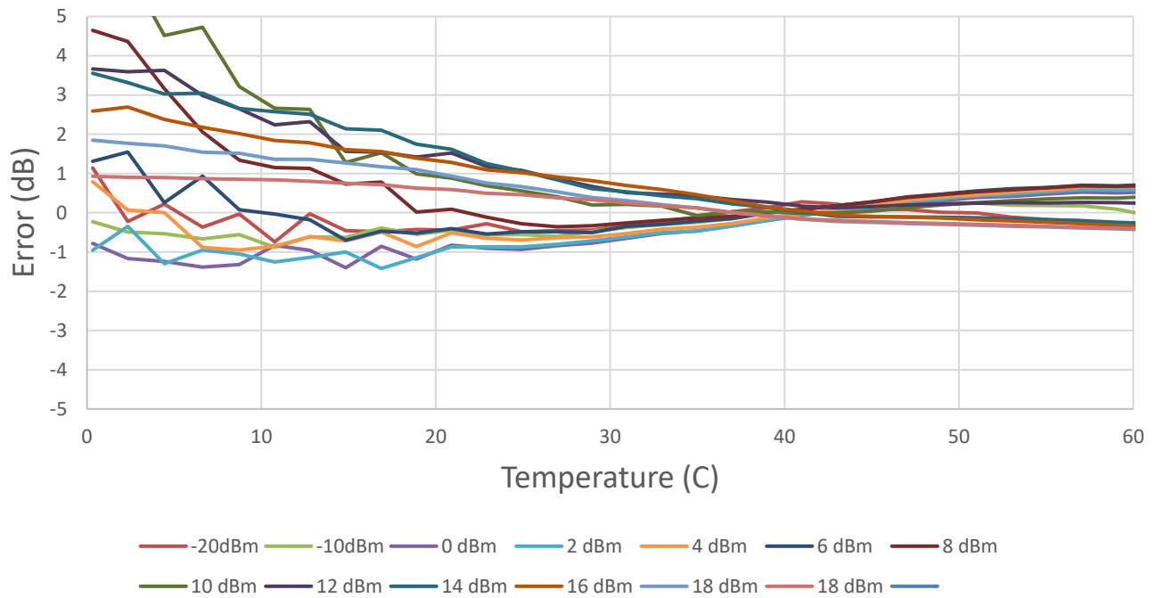
Typical Error vs Temperature vs Power at 1GHz
