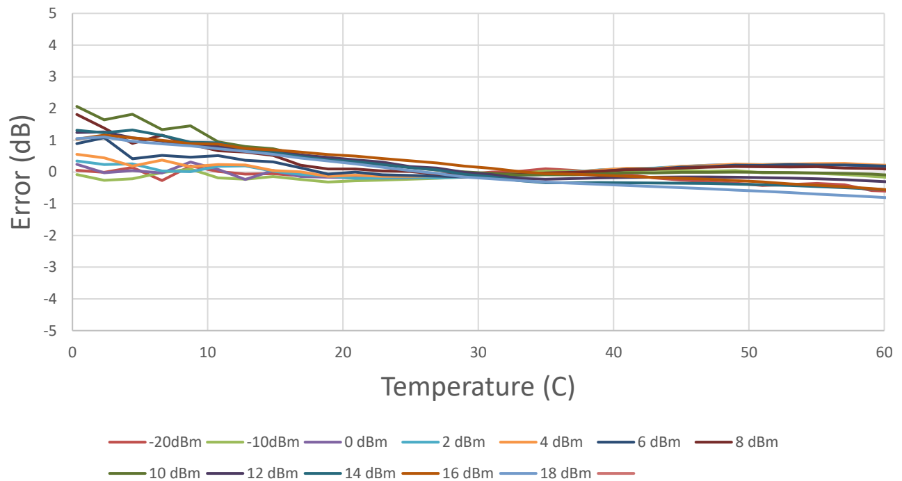
Typical Error vs Temperature vs Power at 5GHz
